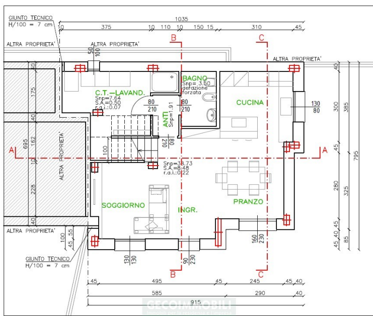
PIANO TERRA
