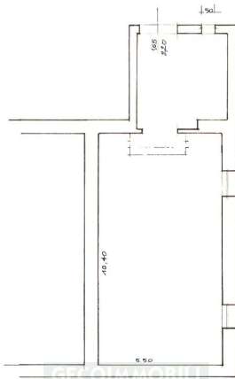
PIANO INTERRATO
