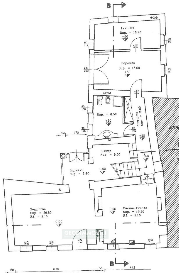
PIANO TERRA
