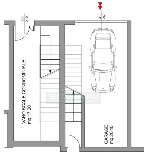
PIANO INTERRATO
