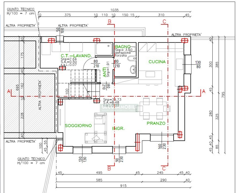
PIANO TERRA
